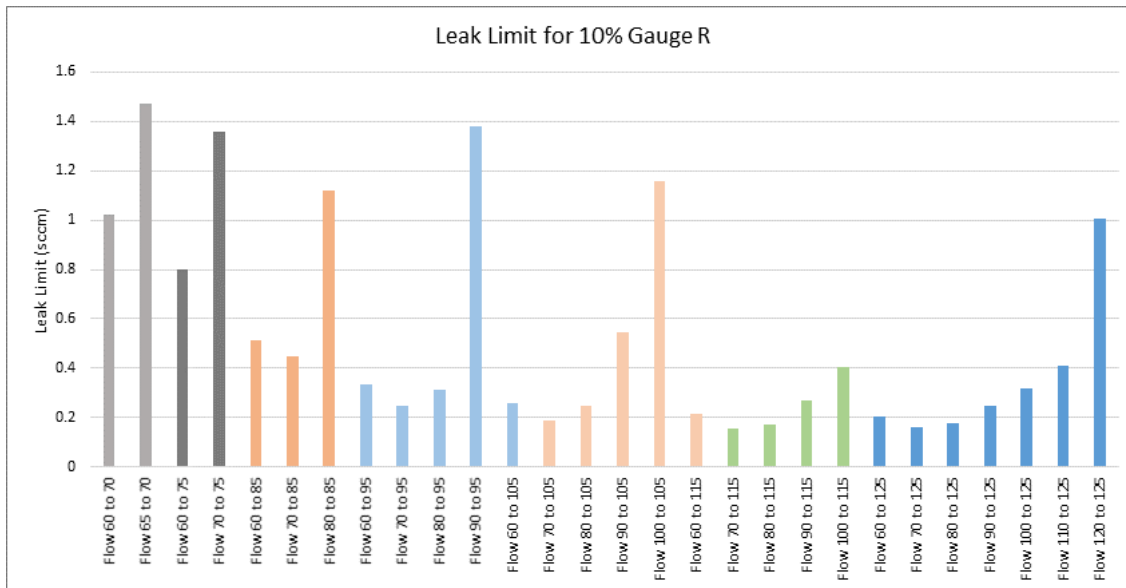
Figure 1 - This graph, produced using Sciometric's QualityWorX data analysis tools, shows a comparison of leak rate vs. gauge R with gauge R constant at 10%. This data enabled the manufacturer to clearly see the impact of shortening cycle time and how it would affect the leak rate and the gauge R.
